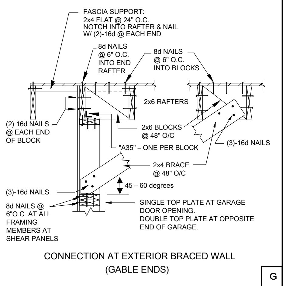
CONNECTION AT EXTERIOR BRACED WALL (RAFTER EAVES) 1 F
