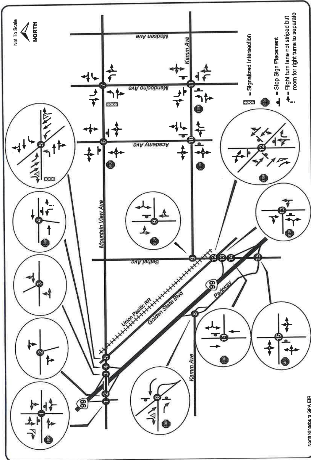
Figure IV-3 Intersection Geometrics and Control
